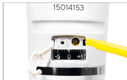
Calibration Adjustment
